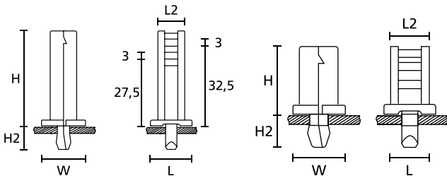
TY5K2 Rivet Mount
